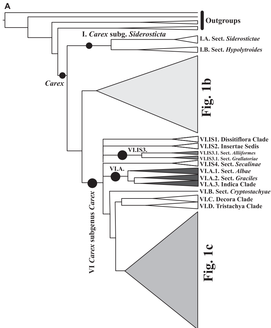
Fig. 1. Phylogenetic scaffold for the Carex classification based on a composite understanding of lineages (Jiménez-Mejías et al., 2016a; Martín-Bravo et al., 2019; Villaverde et al., 2020). A , Root, early branching events in Carex , Carex subgenus Siderosticta , and early branching events in Carex subgenus Carex . B , Carex subgenera Euthyceras , Psyllophorae , Uncinia , and Vigna . C , Carex subgenus Carex . Roman numeral/letter/number combinations refer to recognized sections/clades in the classification. Black dots on internal branches marked with Roman numeral/letter designations are clades recognized in the classification where subclades are recognized. To make it easier to visually recognize named subclades within clades, subclades are given the same gray shading to visually contrast the subclades recognized within clades with other clades. “E–P Clade” = Euthyceras – Psyllophorae Clade, “V–U Clade” = Vigna – Uncinia Clade.
