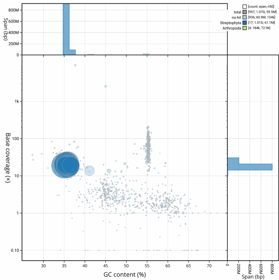
Figure 6. BlobToolKit blob plot for daCirDiss1.hap1.1, the haplotype 1 assembly. The plot shows base coverage (vertical axis) and GC content (horizontal axis). Circles represent scaffolds; marker area is proportional to scaffold length, and colour indicates taxonomic assignment. The histograms along the axes display the total length of sequences distributed across different levels of coverage and GC content. The assembly can be explored interactively in the BlobToolKit viewer .
