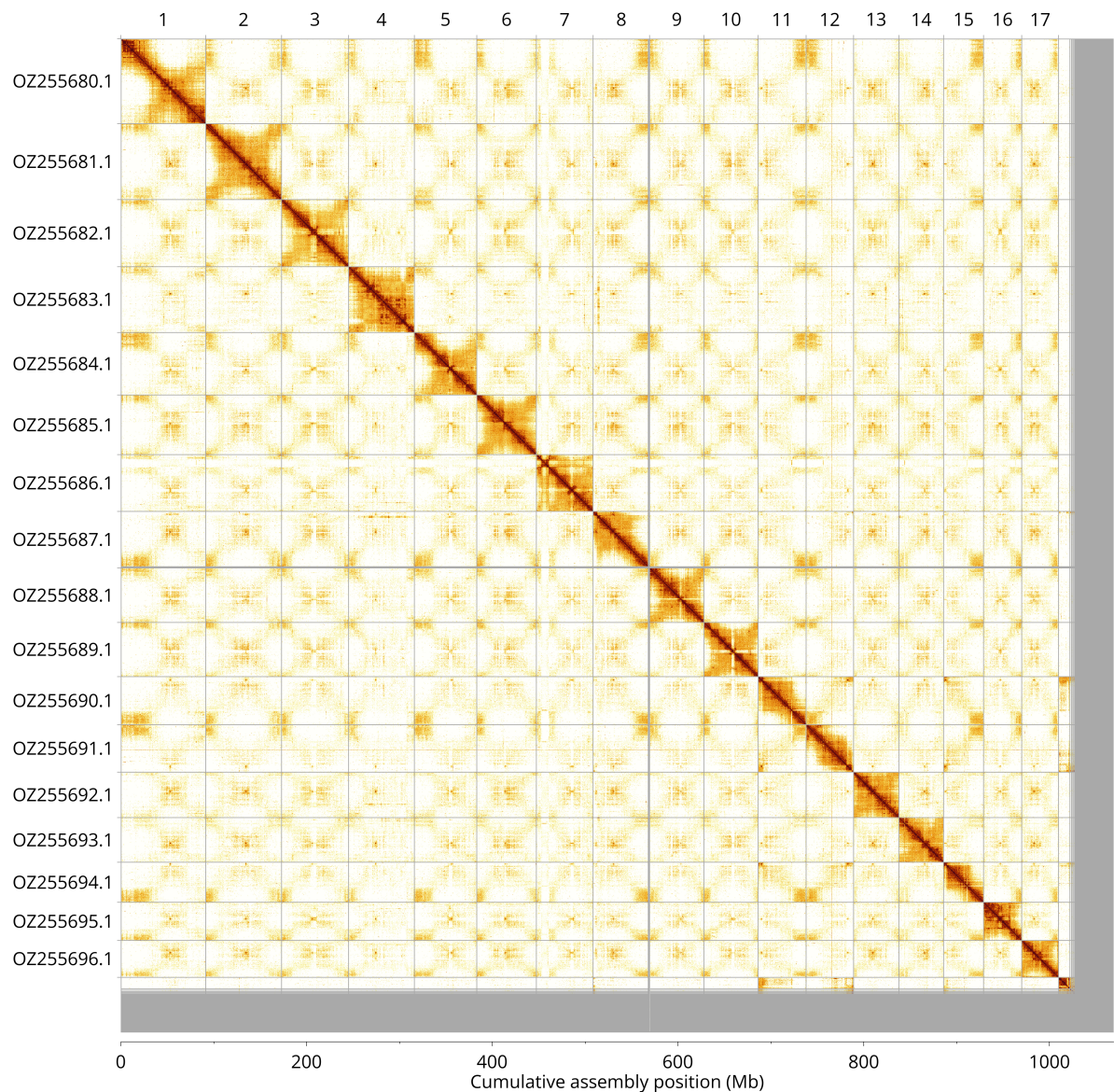
Figure 3. Hi-C contact map of the C. dissectum haplotype 1 assembly. Assembled chromosomes are shown in order of size and labelled along the axes, with a megabase scale shown below. The plot was generated using PretextSnapshot.
