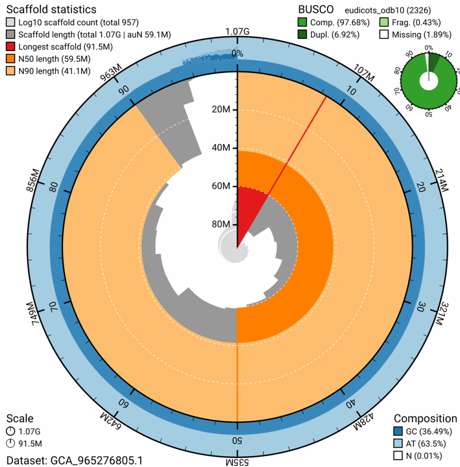
Figure 5. Assembly metrics for daCirDiss1.hap1.1, the haplotype 1 assembly. The BlobToolKit snail plot provides an overview of assembly metrics and BUSCO gene completeness. The circumference represents the length of the haplotype 1 assembly, and the main plot is divided into 1,000 bins around the circumference. The outermost blue tracks display the distribution of GC, AT, and N percentages across the bins. Scaffolds are arranged clockwise from longest to shortest and are depicted in dark grey. Scaffold length is shown on a linear radial scale, scaled to the longest scaffold. Red shading indicates the longest scaffold, and the deeper orange and pale orange shading represent the N50 and N90 lengths. The summary statistics include scaffold auN, the area under the scaffold Nx curve. The light grey spiral at the centre shows the cumulative scaffold count on a logarithmic scale. A summary of complete, fragmented, duplicated, and missing BUSCO genes in the eudicots_odb10 set is presented at the top right. The assembly can be explored interactively in the BlobToolKit viewer .
